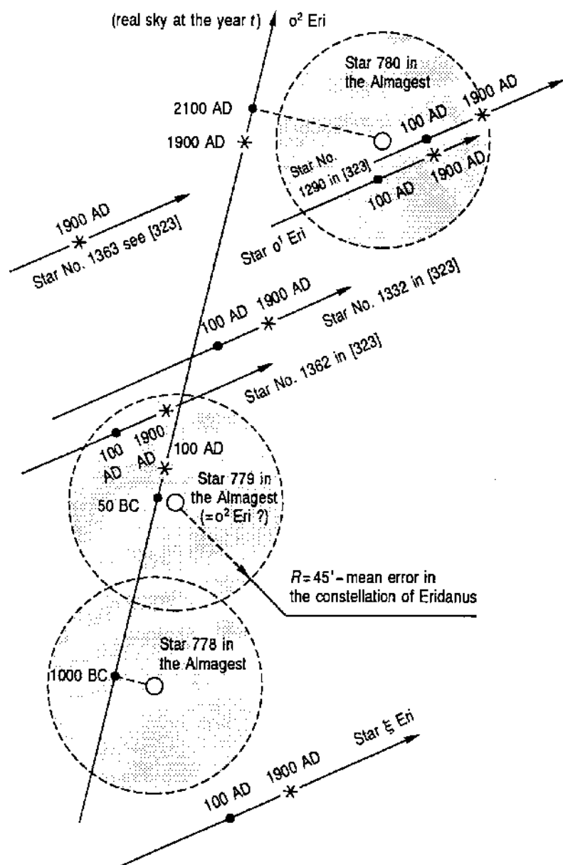
Figure 20(5). The real motion of the stars o^2 Eridanus, No. 1362, No. 1332, No. 1290, No. 1363 (numeration according to D. Hoffleit [323]) and the position of the stars numbered in the Almagest as 778, 779, 780 (according to the Almagest).
