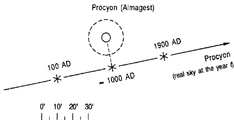
Figure 20(3). The real motion of Procyon and its position according to the Almagest.
