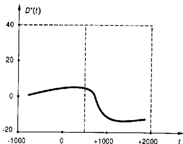
Figure 1. R. Newton's graph demonstrating that D''(t) decreases with time. See the astonishing, inexplicable jump at around the first millennium A.D.
