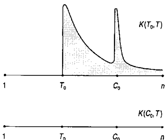
Figure 27. Duplicate-discovery method. The first graph does not satisfy the frequency-damping principle.
