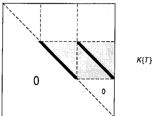
Figure 29. Part of the square frequency matrix for the Bible. Duplicates: (1-2 Samuel + 1-2 Kings) and 1-2 Chronicles.
