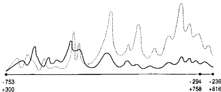
Figure 4. Primary source volume graph, describing ancient (dotted line) and latest (solid line) Roman history: this maximum correlation can hardly be accidental.
