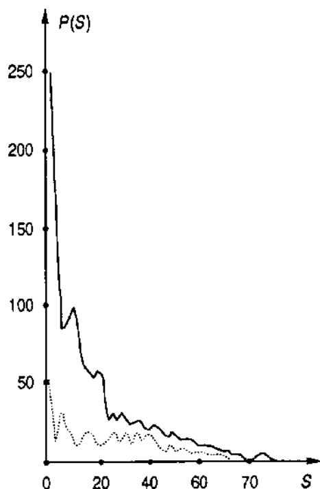
Figure 12. Frequency distribution of the rules of kings of Europe and the Mediterranean region from 3000 B.C. to A.D. 1800 and from A.D. 1400 to 1800
