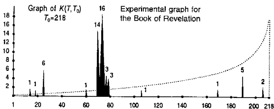
Figure 19. Strong disagreement between the real frequency graph for the Book of Revelation (solid line) and the theoretical frequency graph (dotted line).
