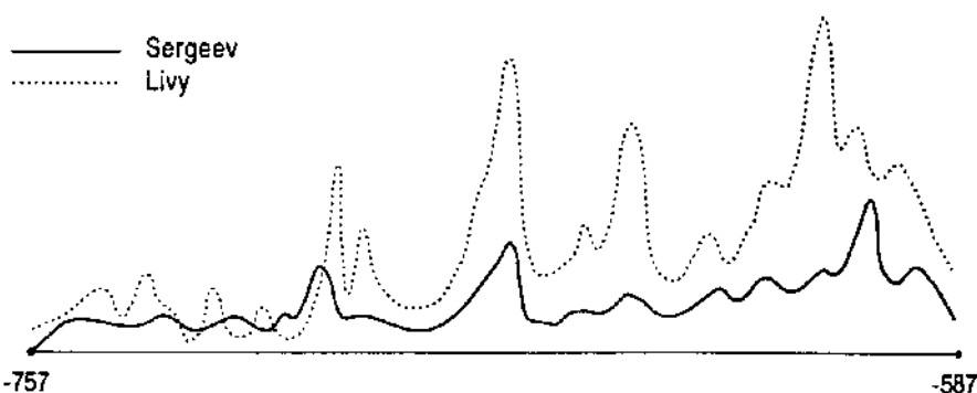
Figure 22. Maximum correlation principle for the volume functions of dependent historical chronicles.
