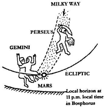
Fig. 3.36. The location of Mars in Gemini, close to Taurus, right under the feet of Perseus, on 1 October 1486.
